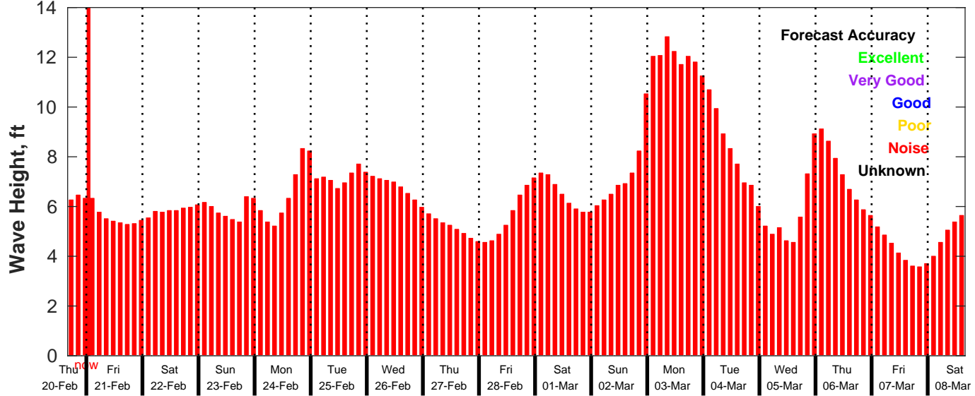
GFS Wave Forecast for NDBC 46069 from 20-Feb-2025 16:00:00 to 08-Mar-2025 16:00:00
