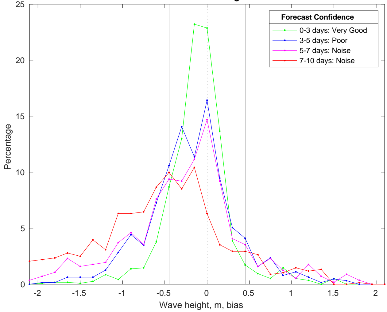
NDBC 46246 vs CMEMS Waves Bias Histogram: 21-Feb-2025
