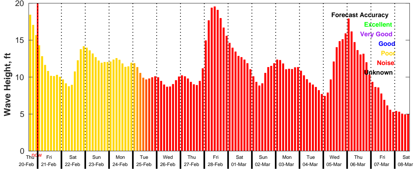
GFS Wave Forecast for NDBC 46246 from 20-Feb-2025 15:00:00 to 08-Mar-2025 15:00:00
