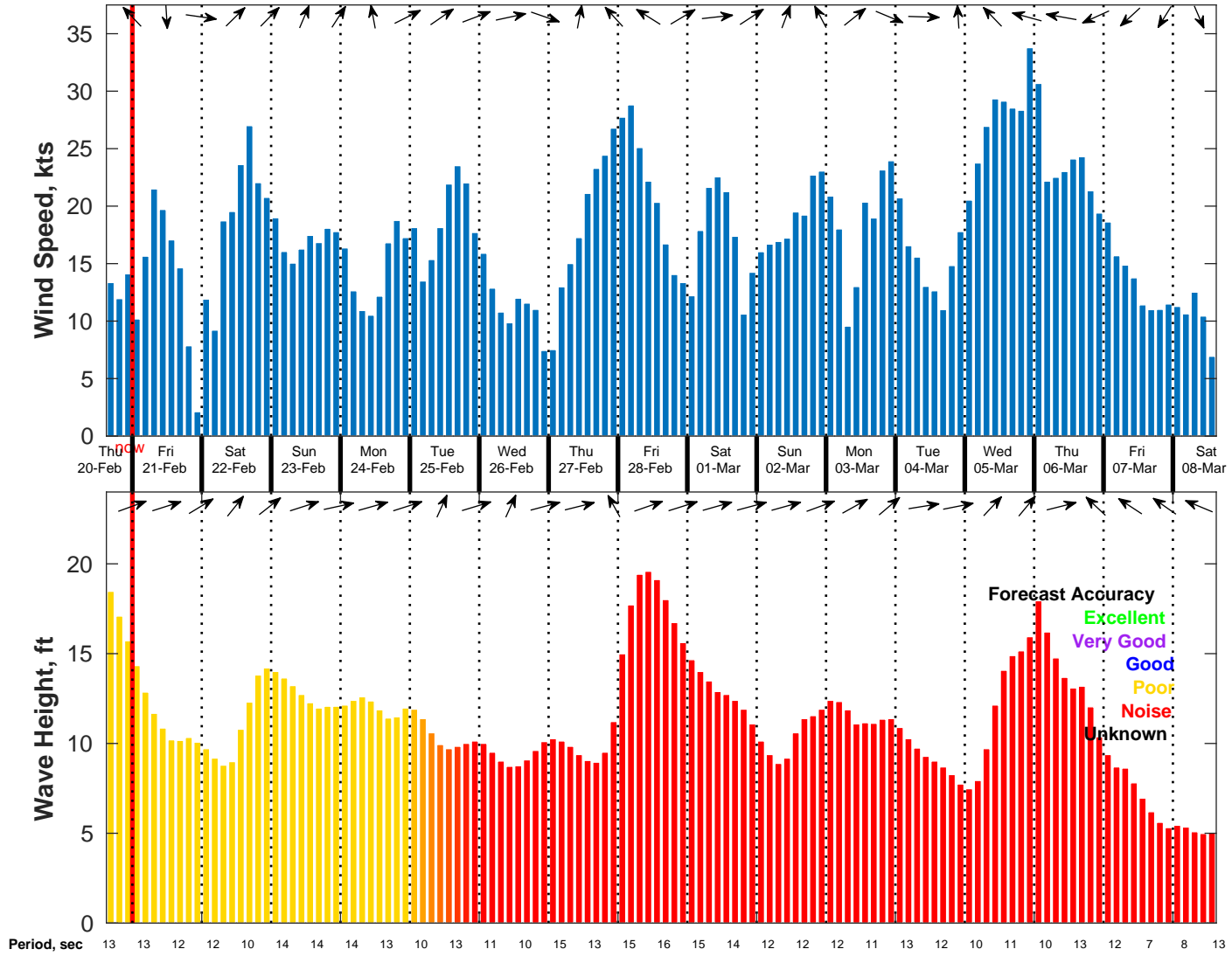
Wind & Wave Forecast for NDBC 46246 from 20-Feb-2025 15:00:00 to 08-Mar-2025 15:00:00
