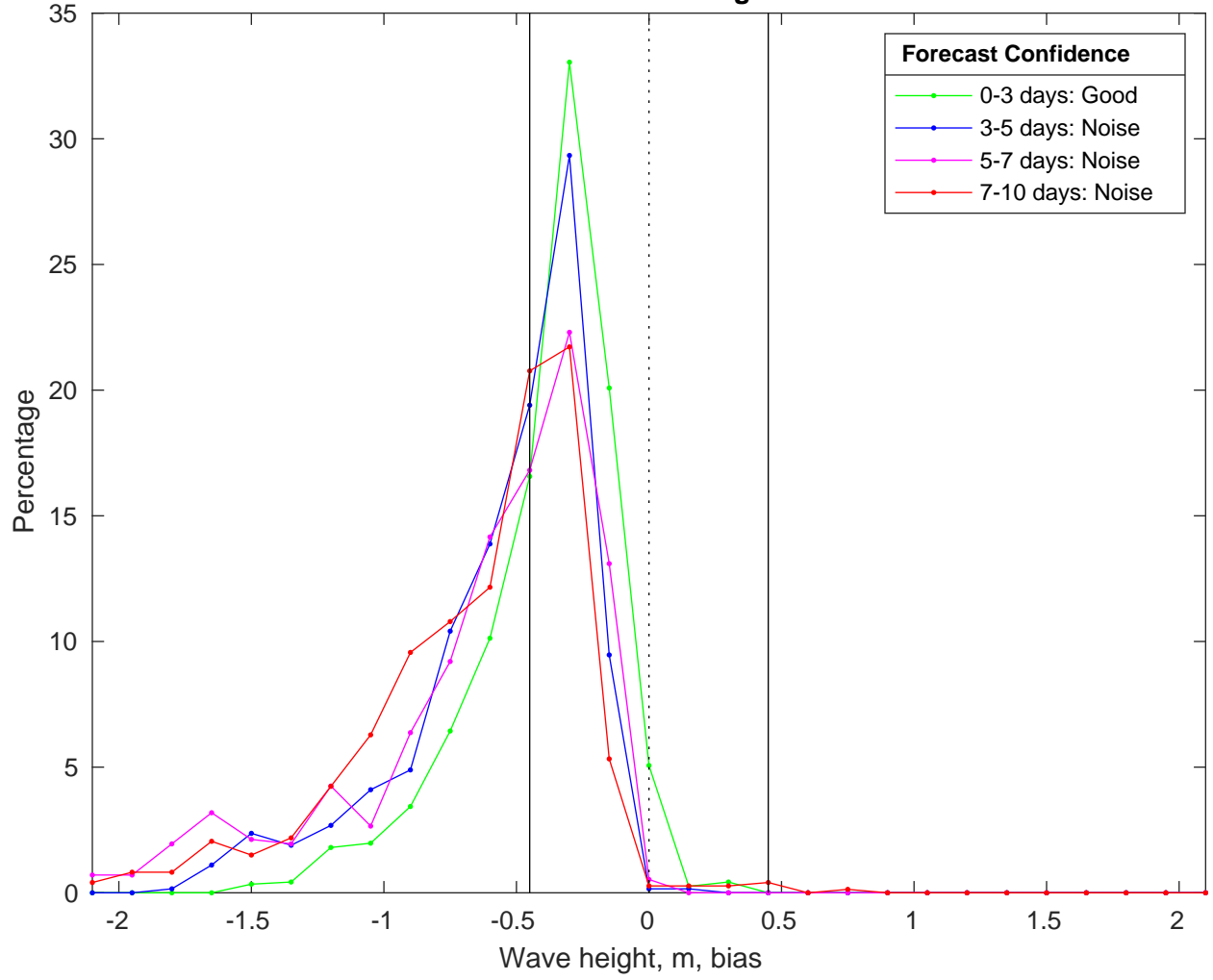
NDBC 51209 vs CMEMS Waves Bias Histogram: 21-Feb-2025
