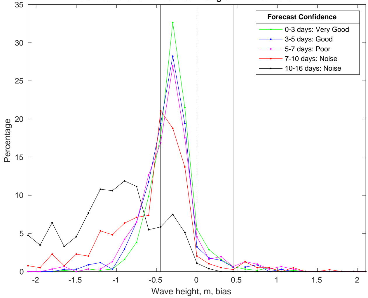
NDBC 51209 vs GFS Waves Bias Histogram: 21-Feb-2025
