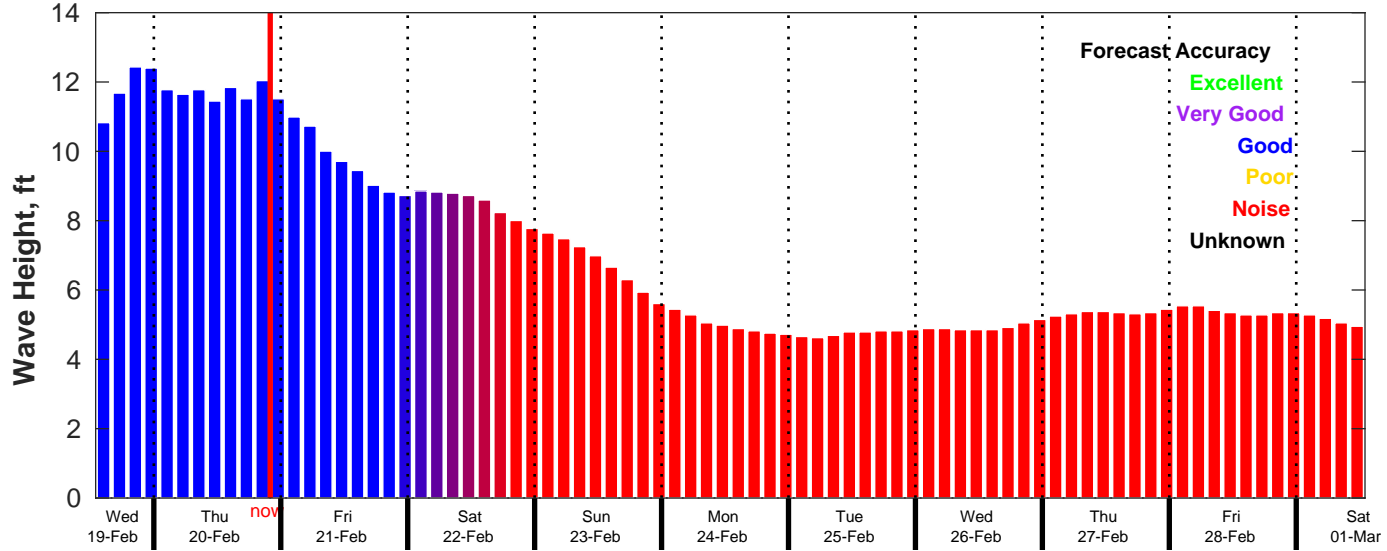
CMEMS Wave Forecast for NDBC 51209 from 19-Feb-2025 13:00:00 to 01-Mar-2025 13:00:00
