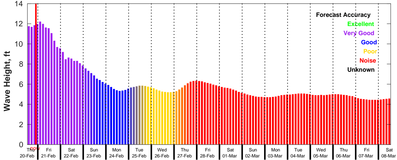
GFS Wave Forecast for NDBC 51209 from 20-Feb-2025 13:00:00 to 08-Mar-2025 13:00:00
