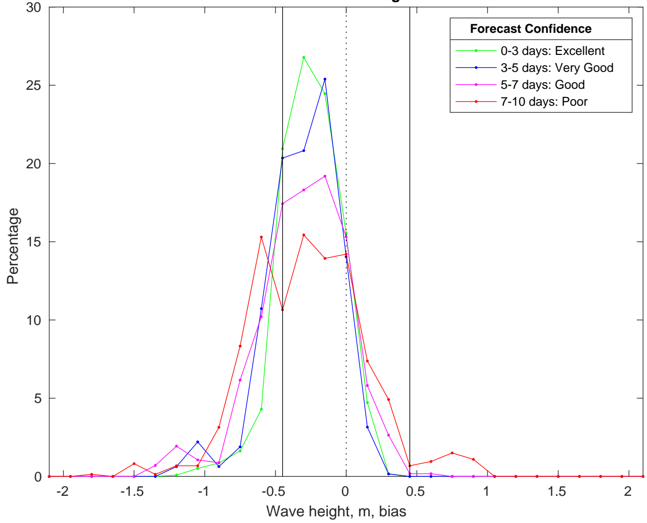
NDBC 52211 vs CMEMS Waves Bias Histogram: 21-Feb-2025
