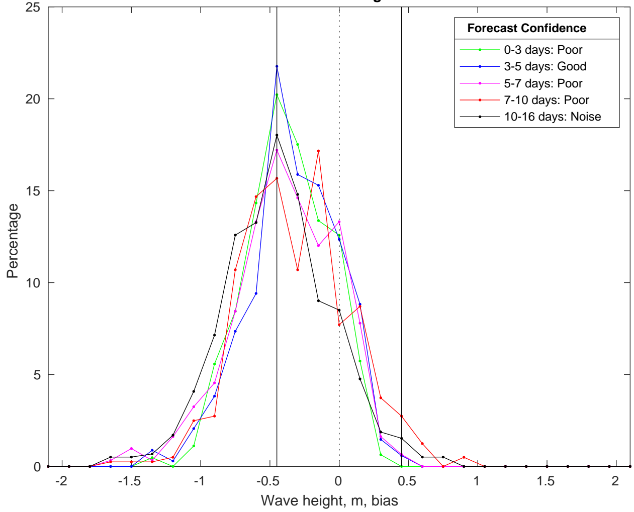
NDBC 52211 vs GFS Waves Bias Histogram: 21-Feb-2025
