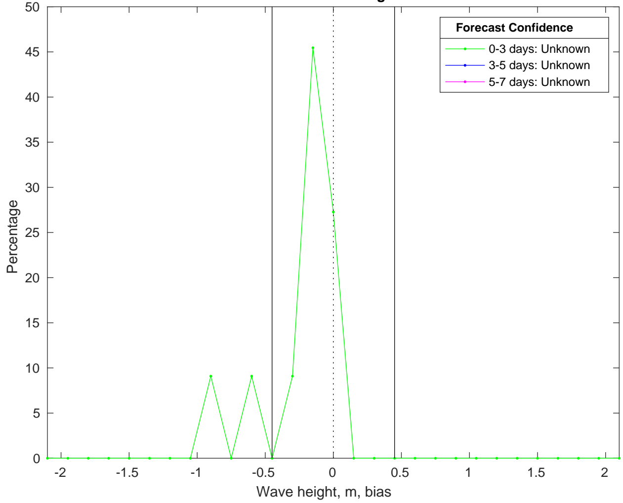
NDBC 52212 vs CMEMS Waves Bias Histogram: 21-Feb-2025
