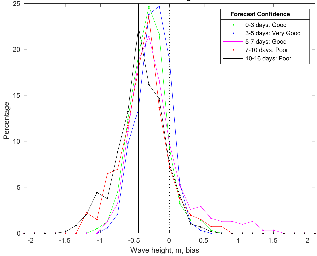
NDBC 52212 vs GFS Waves Bias Histogram: 21-Feb-2025
