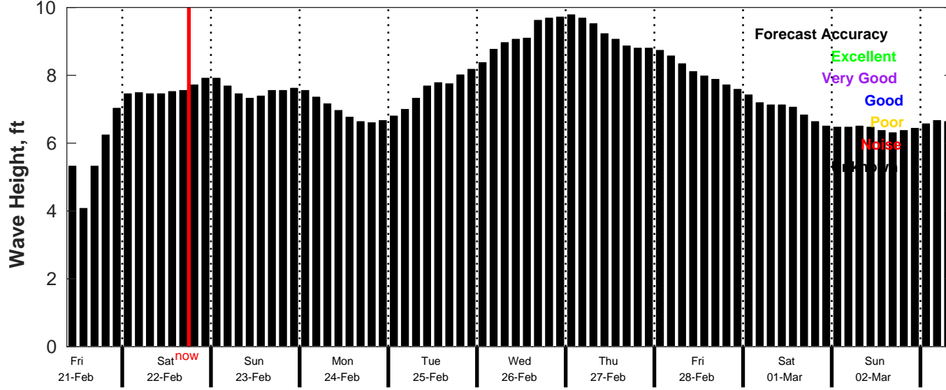
CMEMS Wave Forecast for NDBC 52212 from 20-Feb-2025 09:00:00 to 02-Mar-2025 09:00:00
