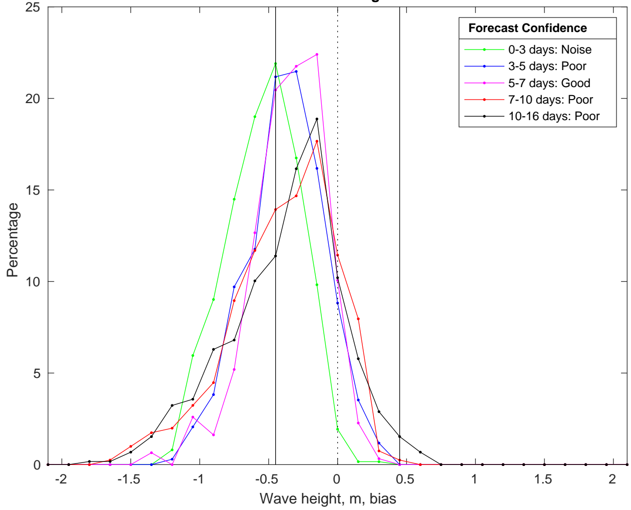
NDBC 52213 vs GFS Waves Bias Histogram: 21-Feb-2025
