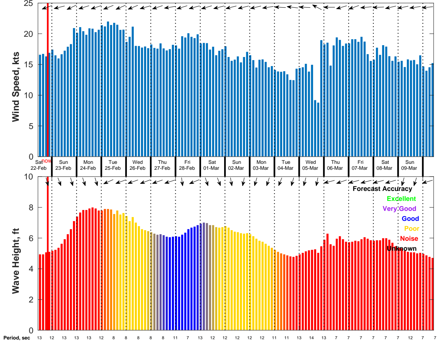
Wind & Wave Forecast for NDBC 52213 from 21-Feb-2025 11:00:00 to 09-Mar-2025 11:00:00
