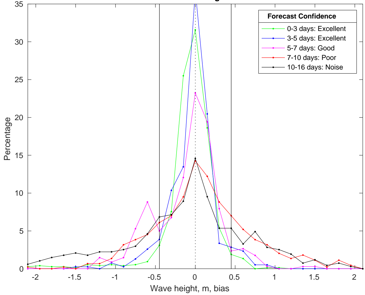
NDBC 41004 vs GFS Waves Bias Histogram: 22-Feb-2025
