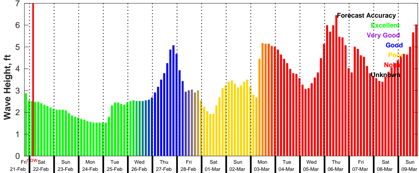
GFS Wave Forecast for NDBC 41004 from 21-Feb-2025 19:00:00 to 09-Mar-2025 19:00:00
