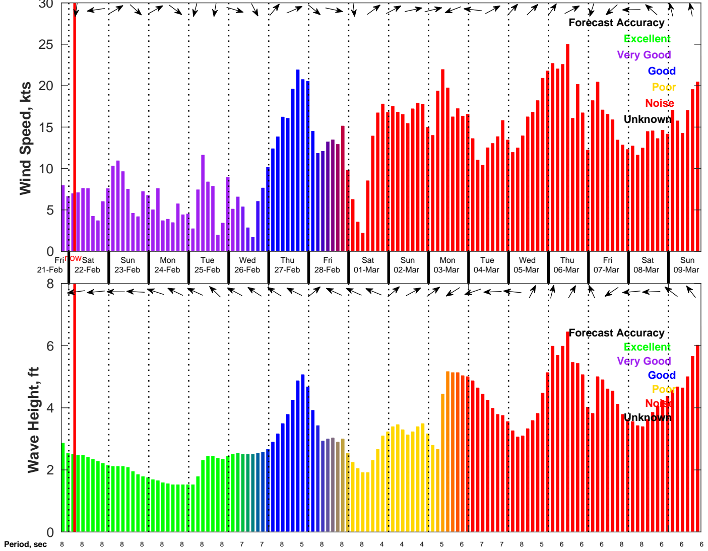
Wind & Wave Forecast for NDBC 41004 from 21-Feb-2025 19:00:00 to 09-Mar-2025 19:00:00
