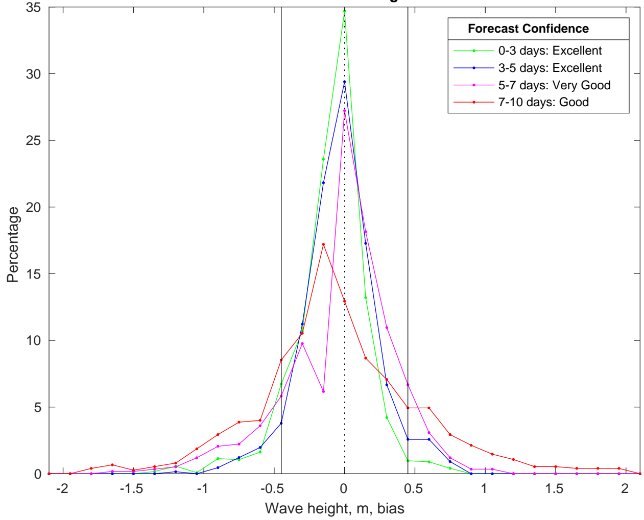
NDBC 41013 vs CMEMS Waves Bias Histogram: 22-Feb-2025
