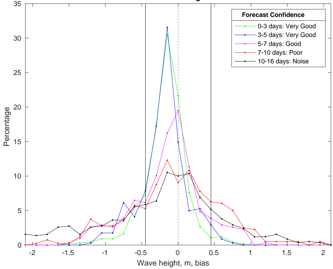
NDBC 41013 vs GFS Waves Bias Histogram: 22-Feb-2025
