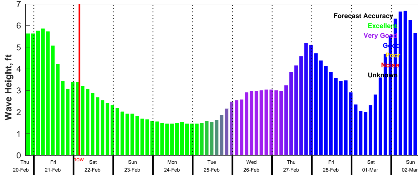
CMEMS Wave Forecast for NDBC 41013 from 20-Feb-2025 19:00:00 to 02-Mar-2025 19:00:00
