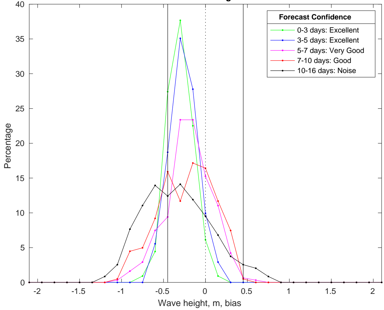
NDBC 41040 vs GFS Waves Bias Histogram: 22-Feb-2025
