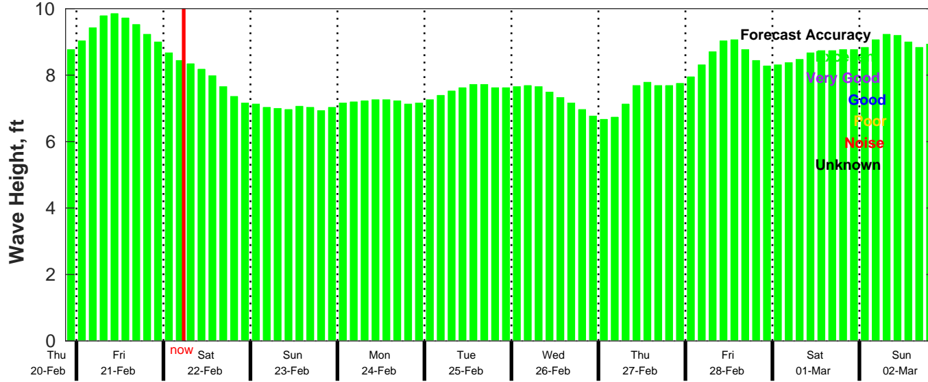
CMEMS Wave Forecast for NDBC 41040 from 20-Feb-2025 21:00:00 to 02-Mar-2025 21:00:00
