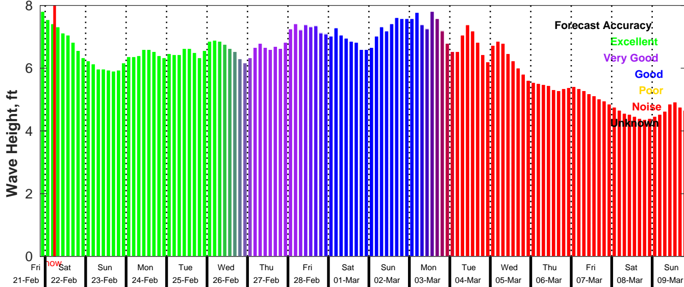
GFS Wave Forecast for NDBC 41040 from 21-Feb-2025 21:00:00 to 09-Mar-2025 21:00:00
