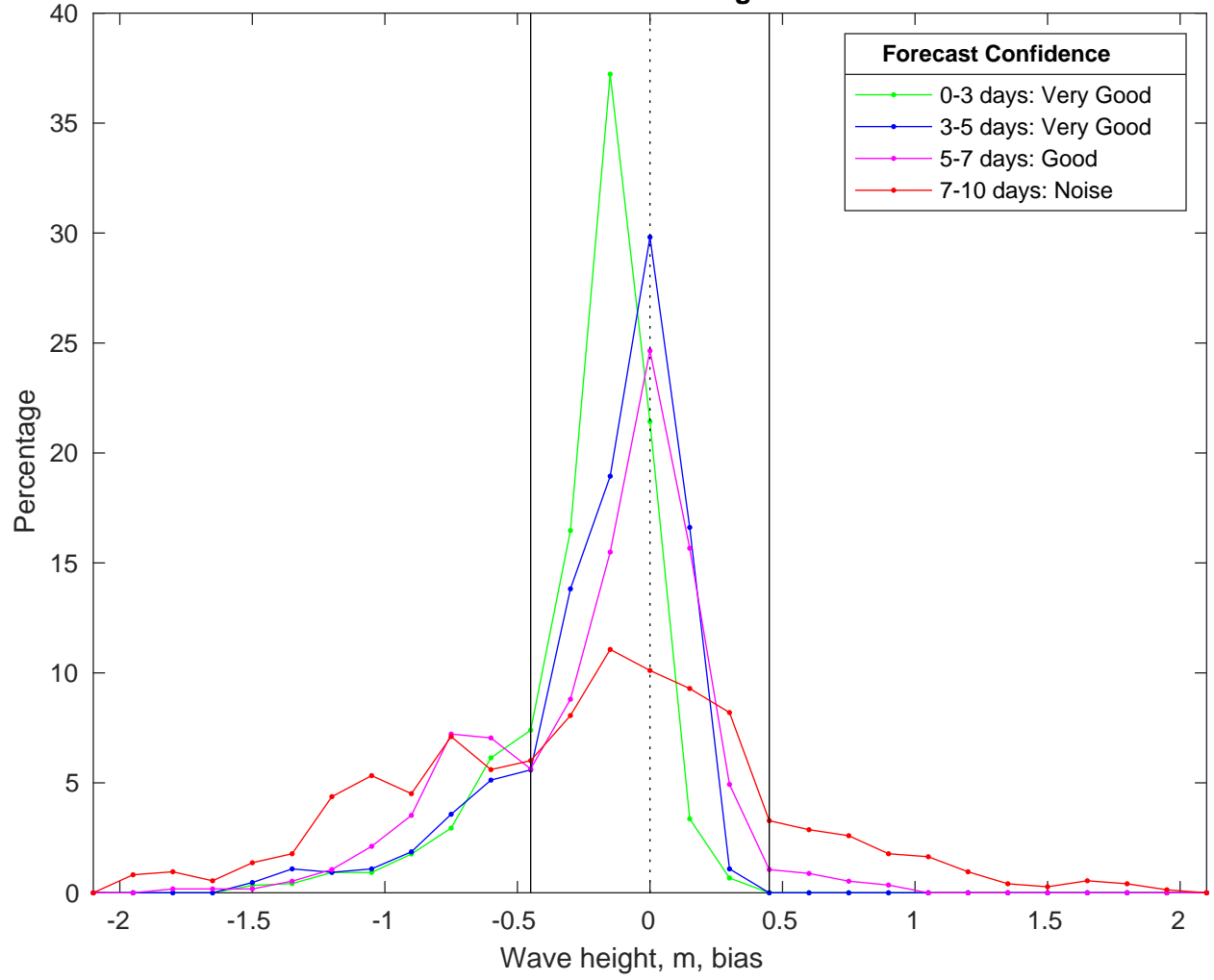
NDBC 42019 vs CMEMS Waves Bias Histogram: 22-Feb-2025
