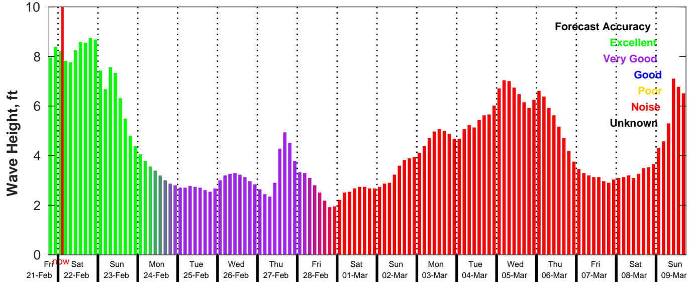
GFS Wave Forecast for NDBC 42019 from 21-Feb-2025 18:00:00 to 09-Mar-2025 18:00:00
