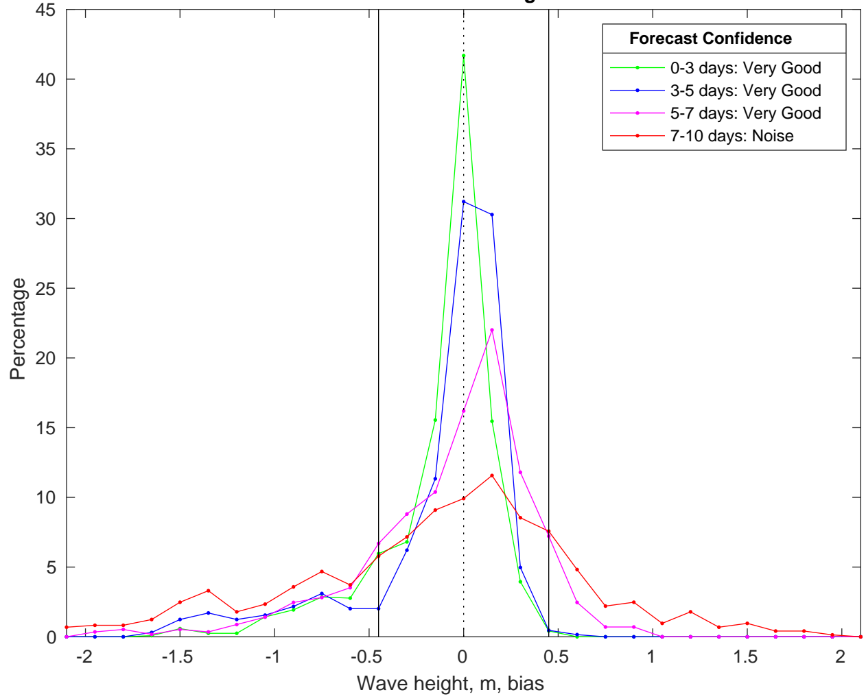
NDBC 42020 vs CMEMS Waves Bias Histogram: 22-Feb-2025
