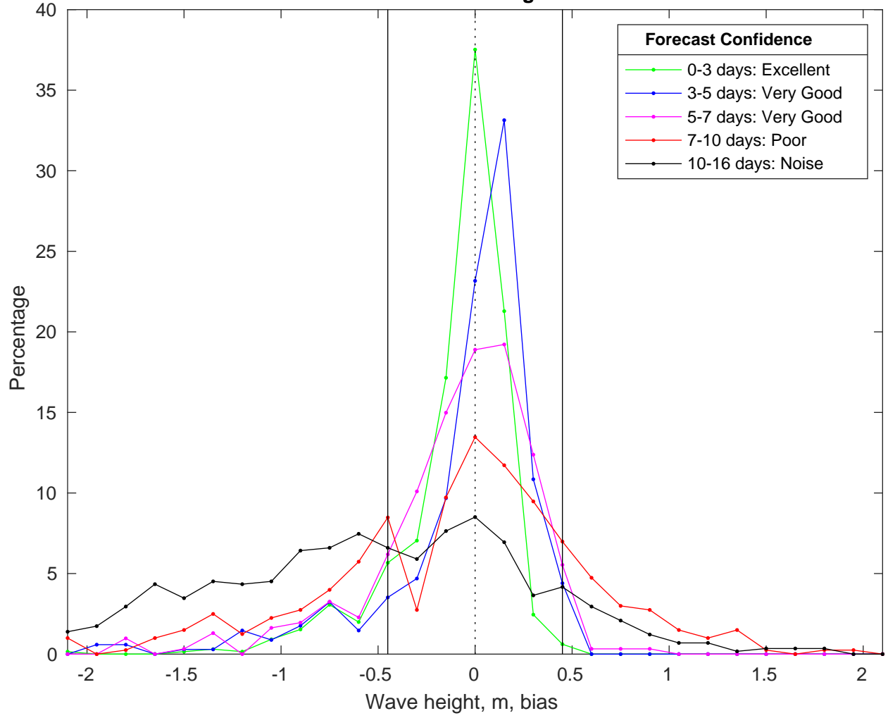
NDBC 42020 vs GFS Waves Bias Histogram: 22-Feb-2025
