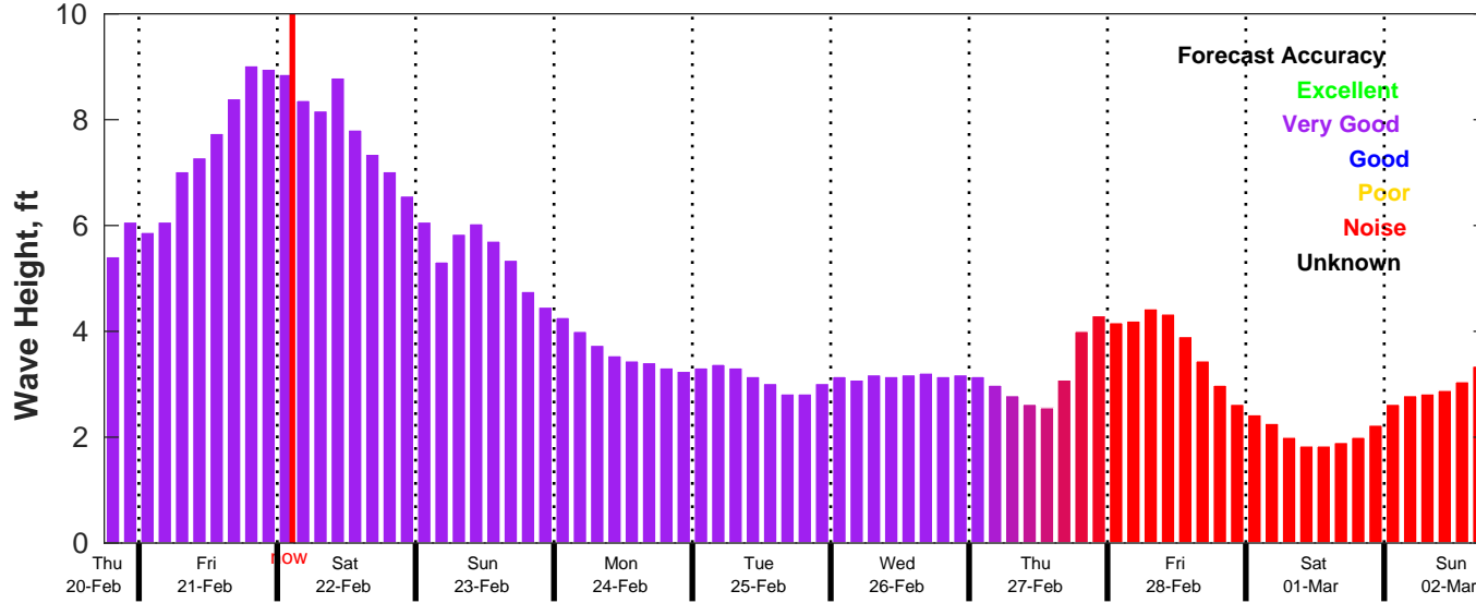
CMEMS Wave Forecast for NDBC 42020 from 20-Feb-2025 18:00:00 to 02-Mar-2025 18:00:00
