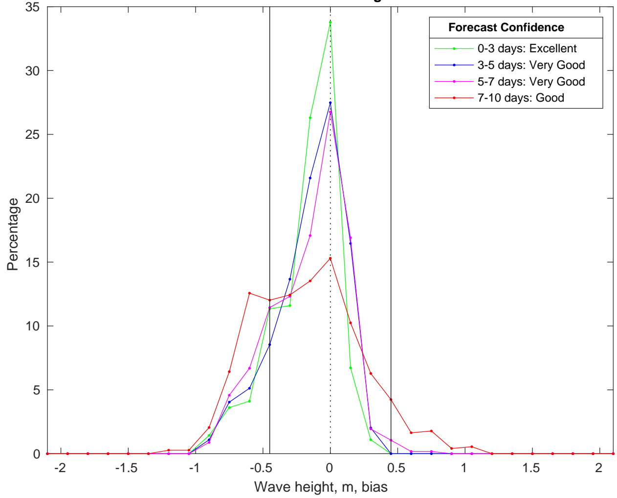
NDBC 42035 vs CMEMS Waves Bias Histogram: 22-Feb-2025
