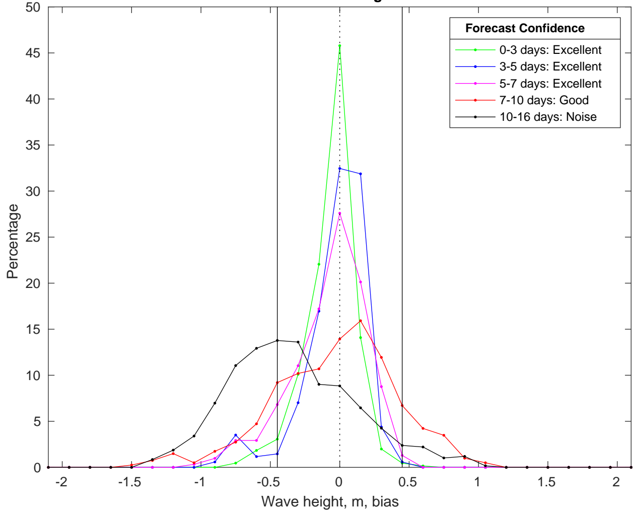
NDBC 42035 vs GFS Waves Bias Histogram: 22-Feb-2025
