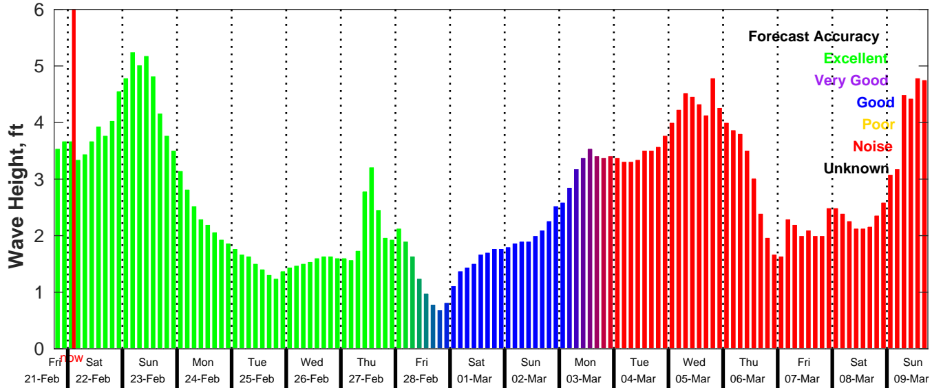
GFS Wave Forecast for NDBC 42035 from 21-Feb-2025 18:00:00 to 09-Mar-2025 18:00:00
