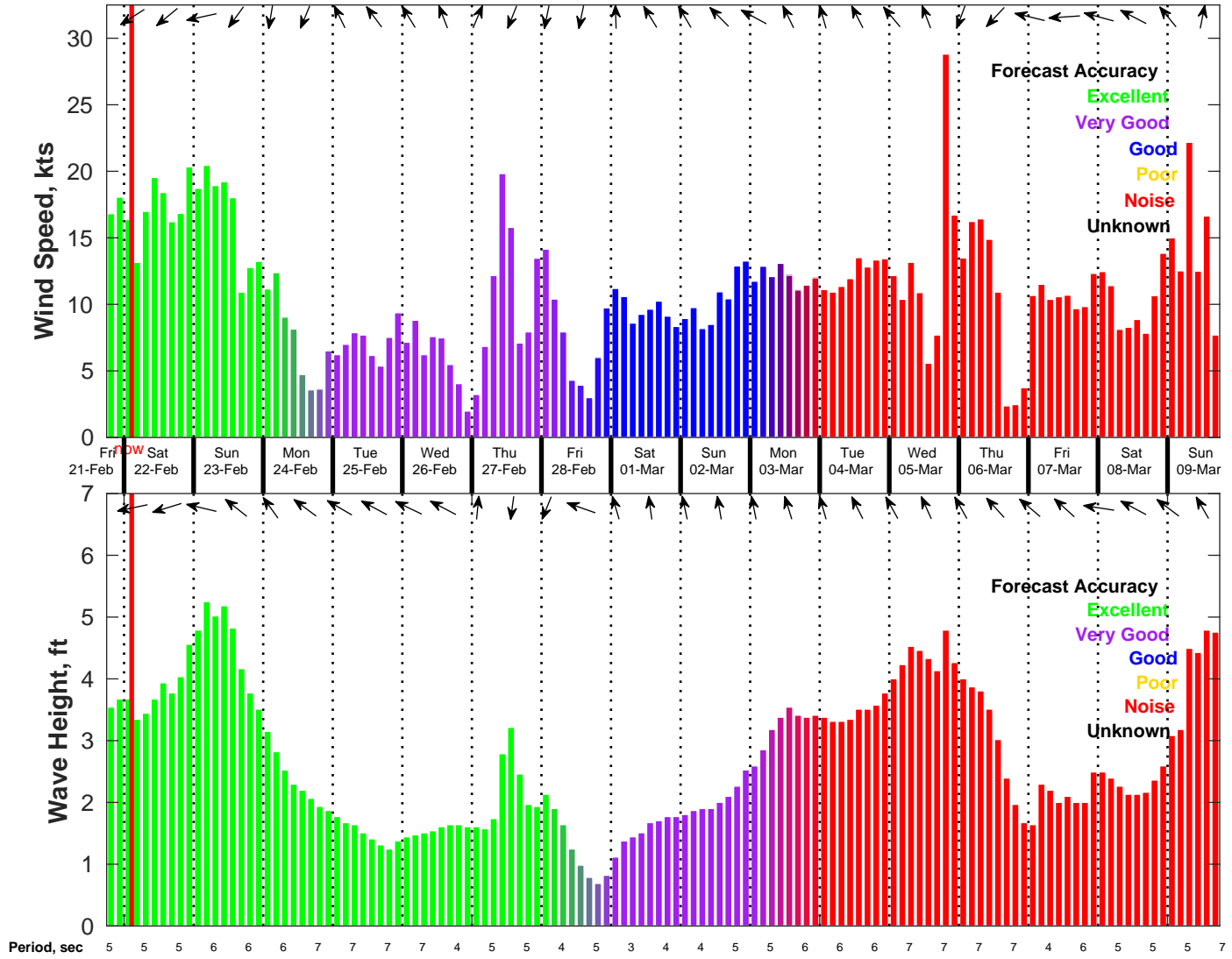
Wind & Wave Forecast for NDBC 42035 from 21-Feb-2025 18:00:00 to 09-Mar-2025 18:00:00
