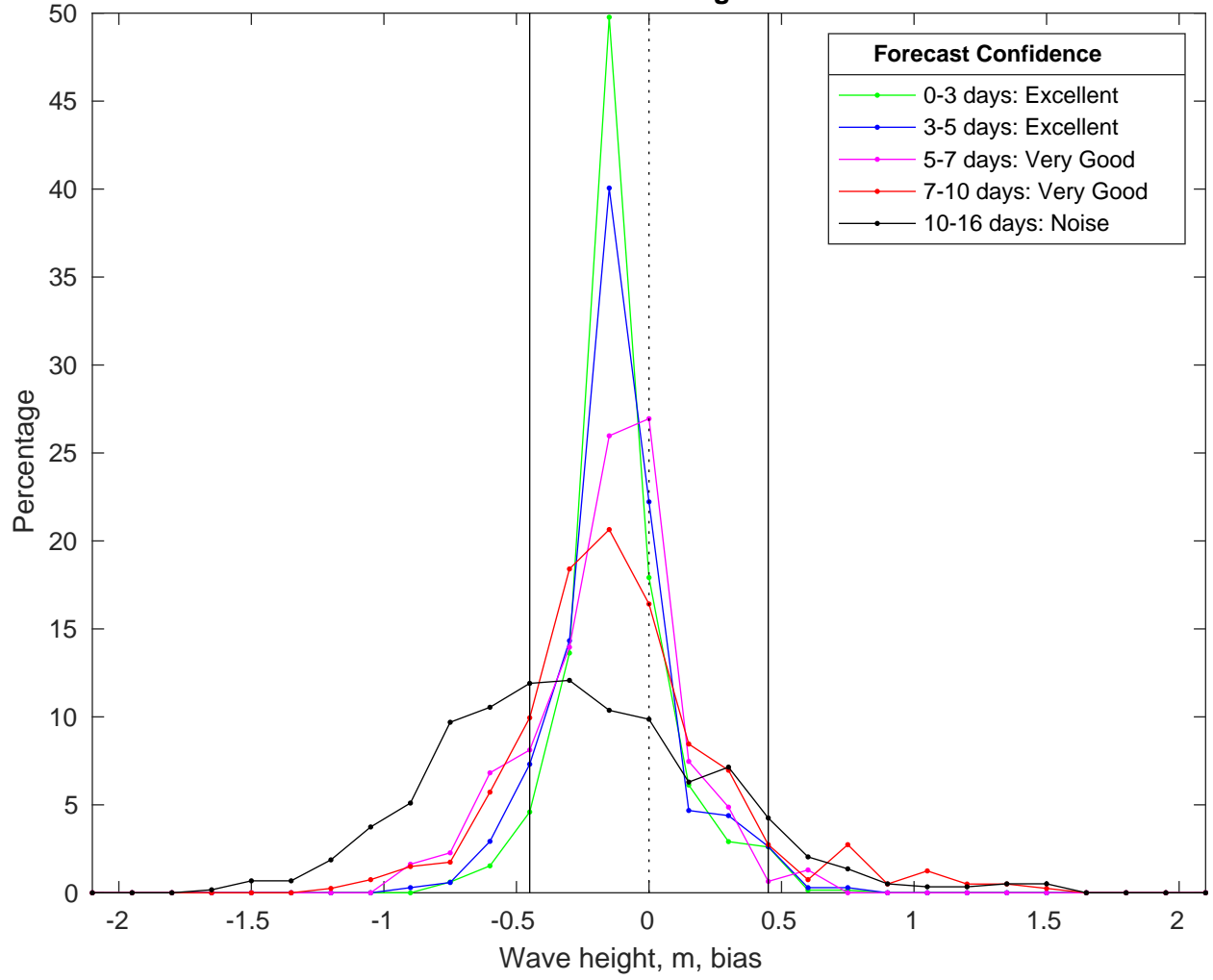
NDBC 42036 vs GFS Waves Bias Histogram: 22-Feb-2025
