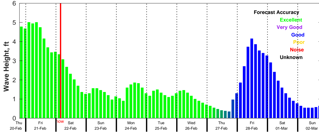
CMEMS Wave Forecast for NDBC 42036 from 20-Feb-2025 19:00:00 to 02-Mar-2025 19:00:00
