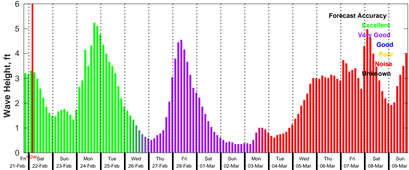
GFS Wave Forecast for NDBC 42036 from 21-Feb-2025 19:00:00 to 09-Mar-2025 19:00:00
