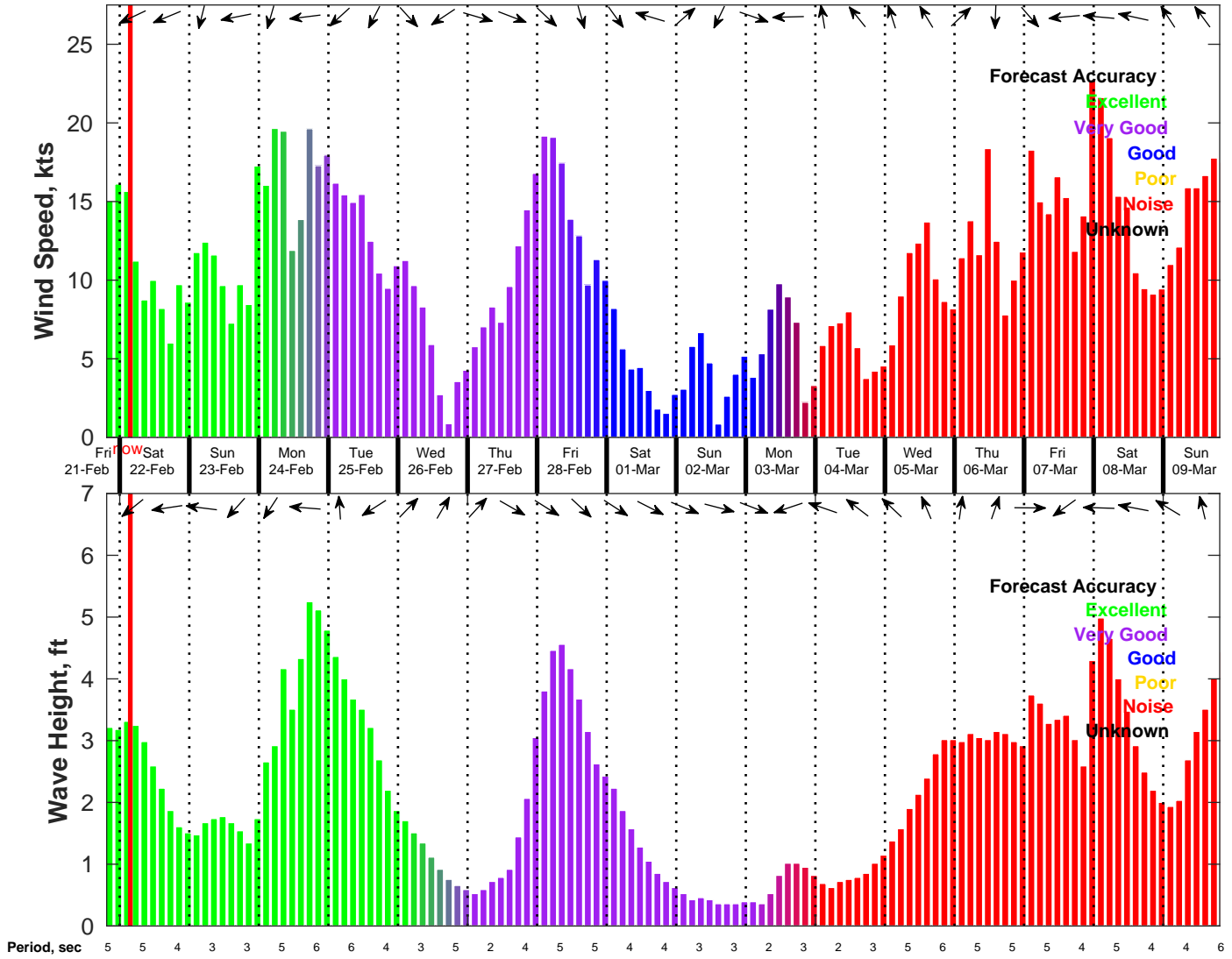
Wind & Wave Forecast for NDBC 42036 from 21-Feb-2025 19:00:00 to 09-Mar-2025 19:00:00
