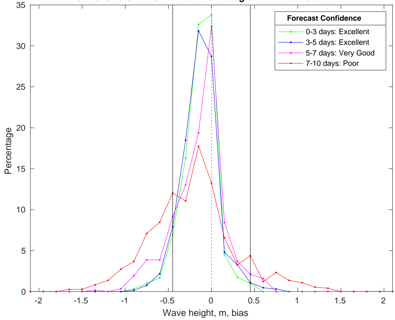
NDBC 42040 vs CMEMS Waves Bias Histogram: 22-Feb-2025
