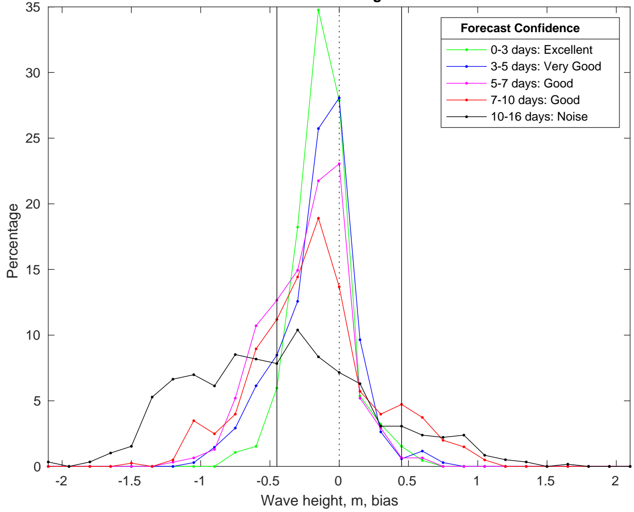
NDBC 42040 vs GFS Waves Bias Histogram: 22-Feb-2025
