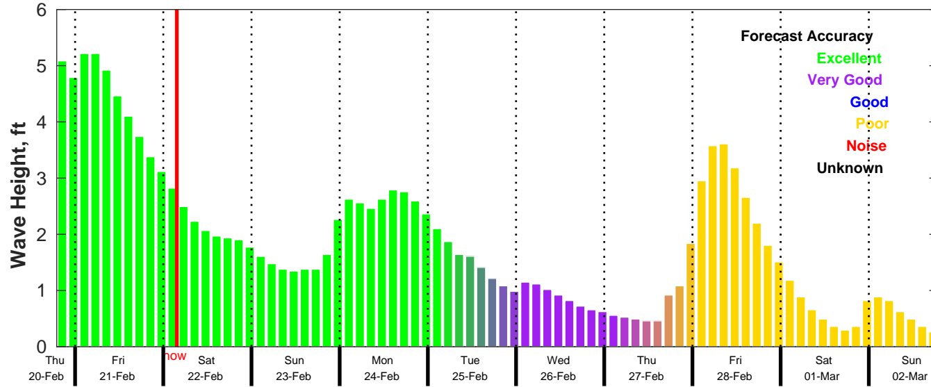
CMEMS Wave Forecast for NDBC 42040 from 20-Feb-2025 19:00:00 to 02-Mar-2025 19:00:00
