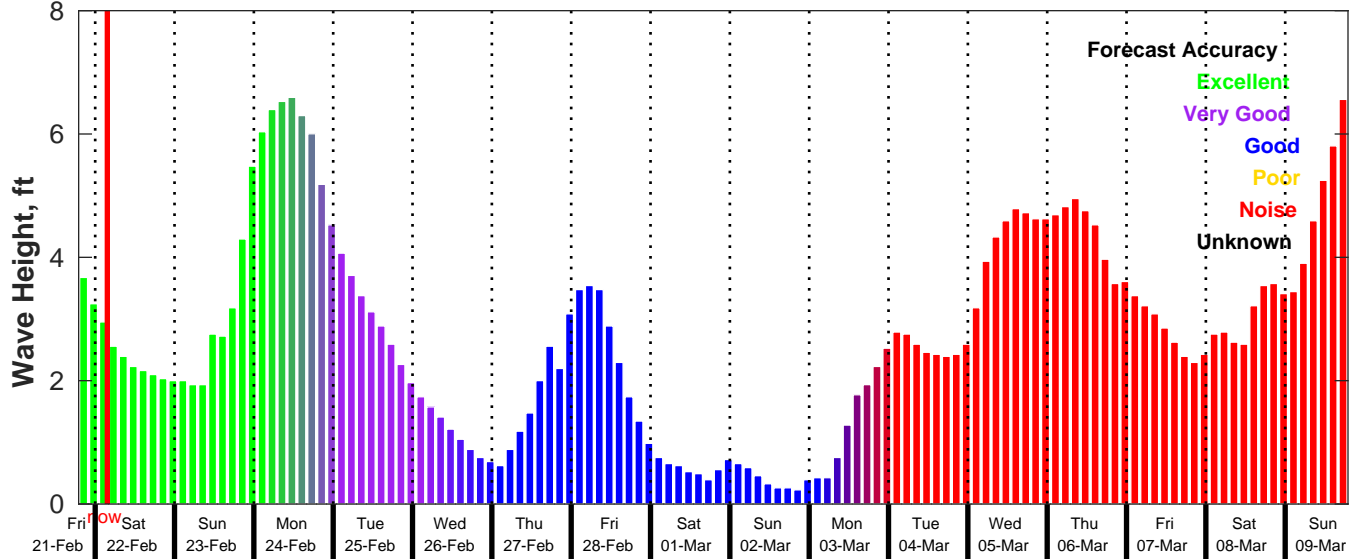
GFS Wave Forecast for NDBC 42040 from 21-Feb-2025 19:00:00 to 09-Mar-2025 19:00:00
