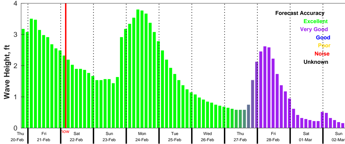
CMEMS Wave Forecast for NDBC 42084 from 20-Feb-2025 19:00:00 to 02-Mar-2025 19:00:00
