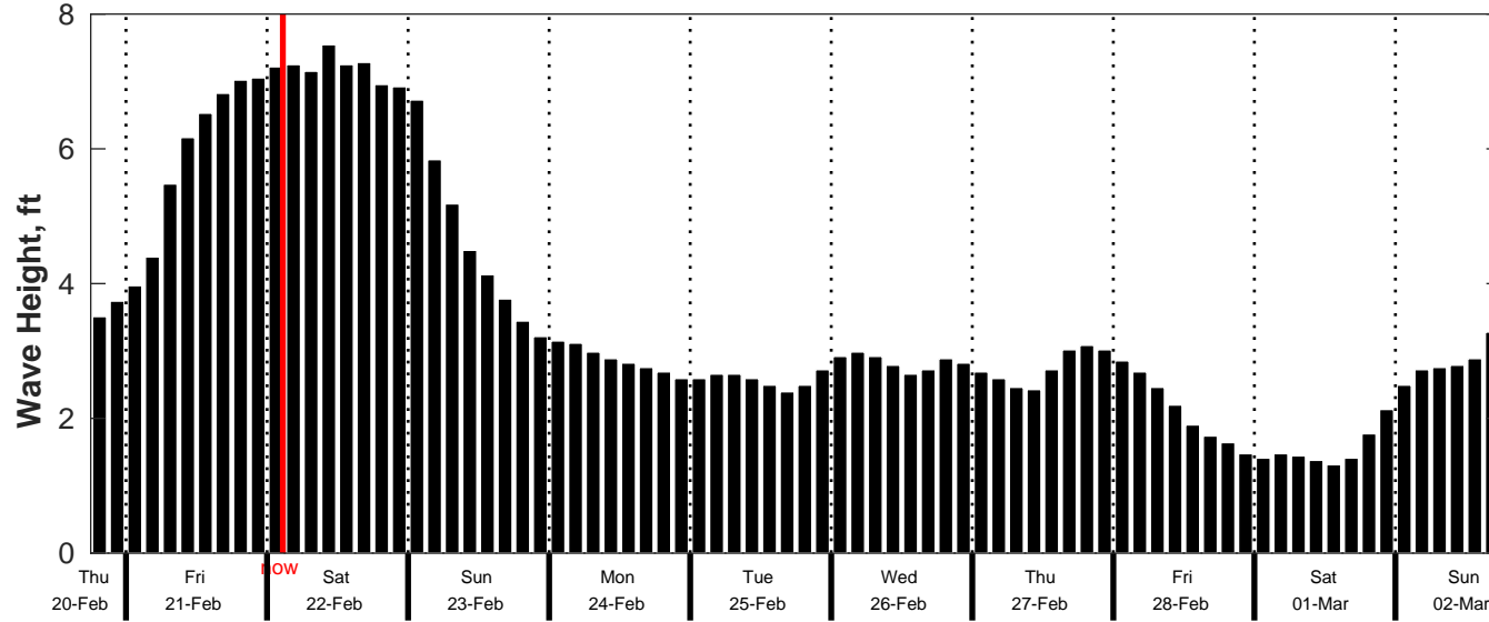
CMEMS Wave Forecast for NDBC 42092 from 20-Feb-2025 18:00:00 to 02-Mar-2025 18:00:00
