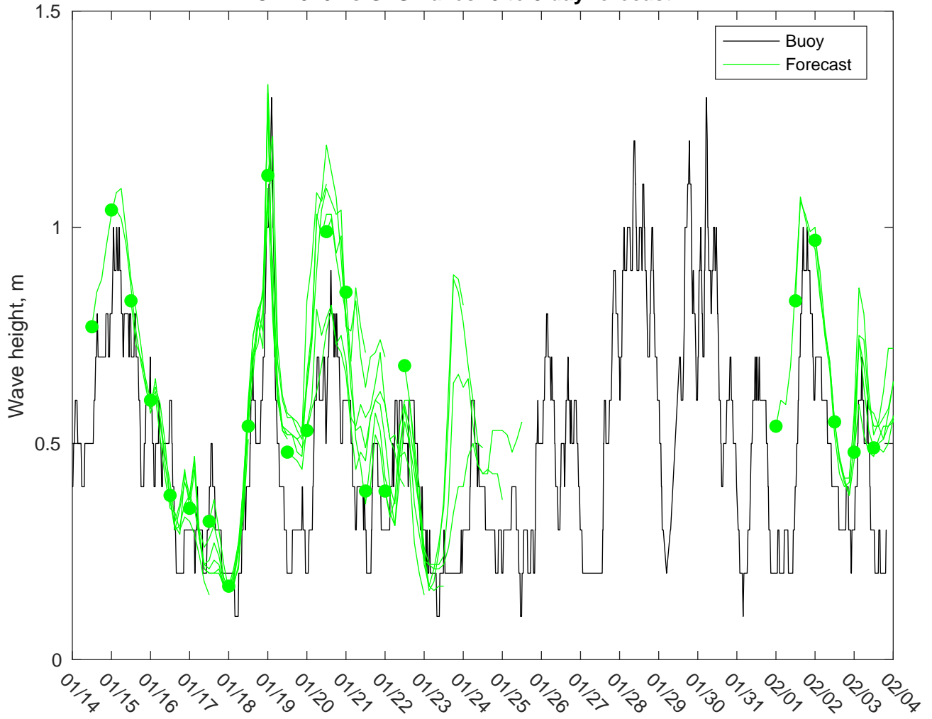
NDBC 44020 vs GFSWaves: 0 to 3 day forecast
