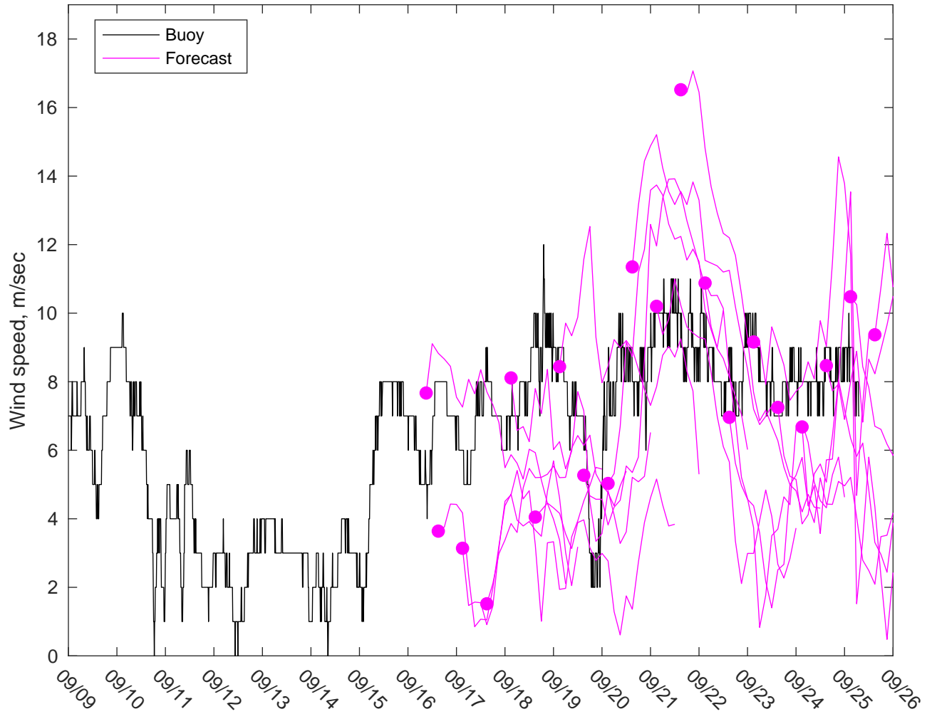
NDBC 44025 vs GFSWinds: 7 to 10 day forecast
