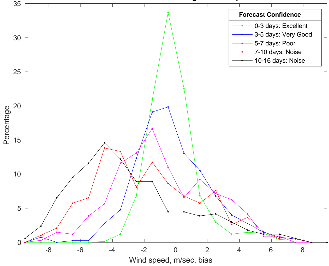
NDBC 44025 vs GFS Winds Bias Histogram: 25-Sep-2024
