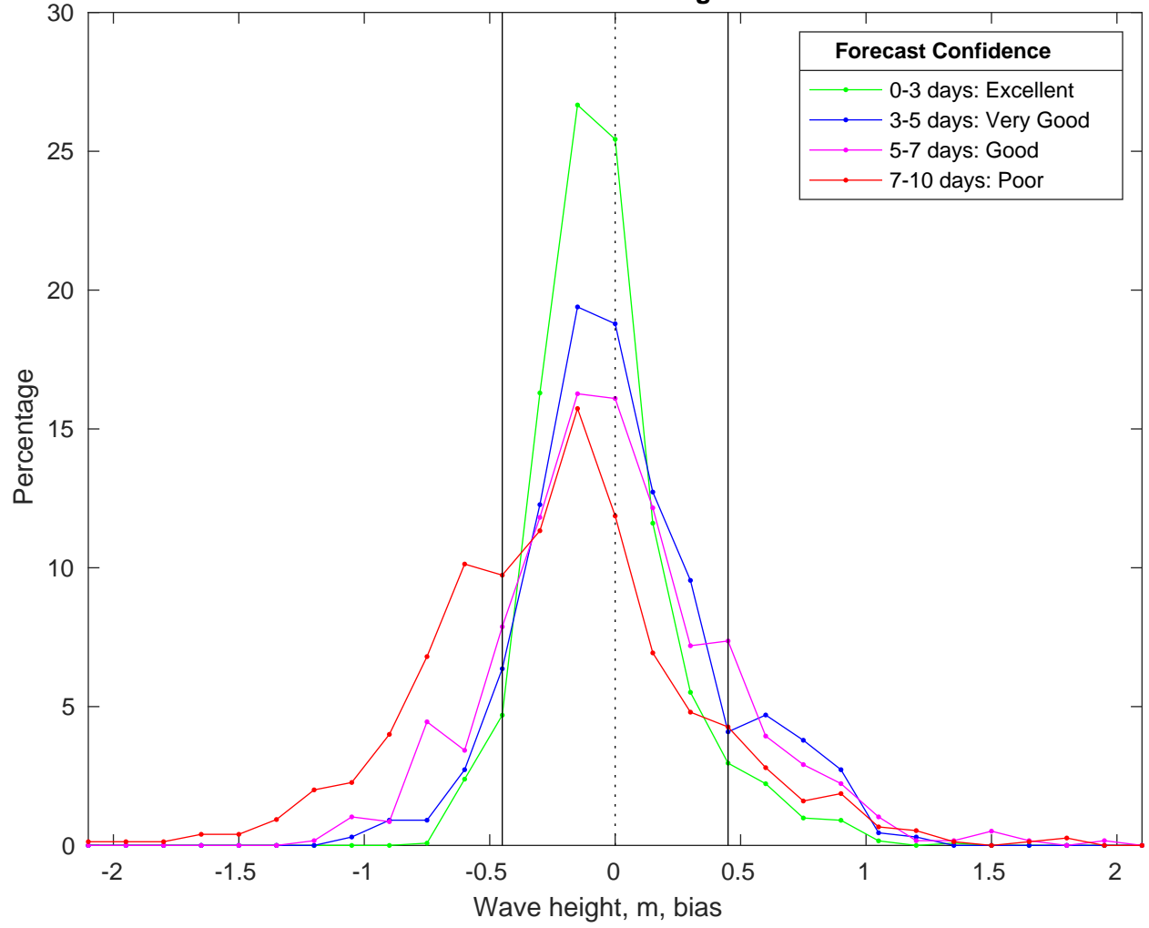
NDBC 46011 vs CMEMS Waves Bias Histogram: 22-Feb-2025
