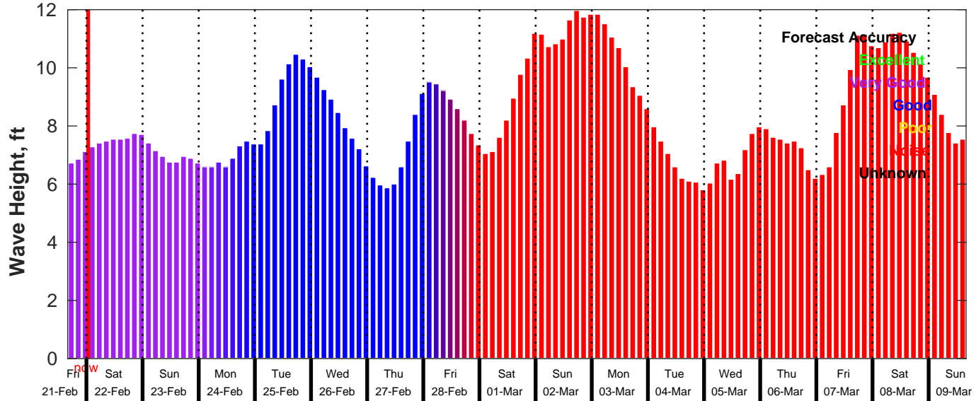
GFS Wave Forecast for NDBC 46011 from 21-Feb-2025 16:00:00 to 09-Mar-2025 16:00:00
