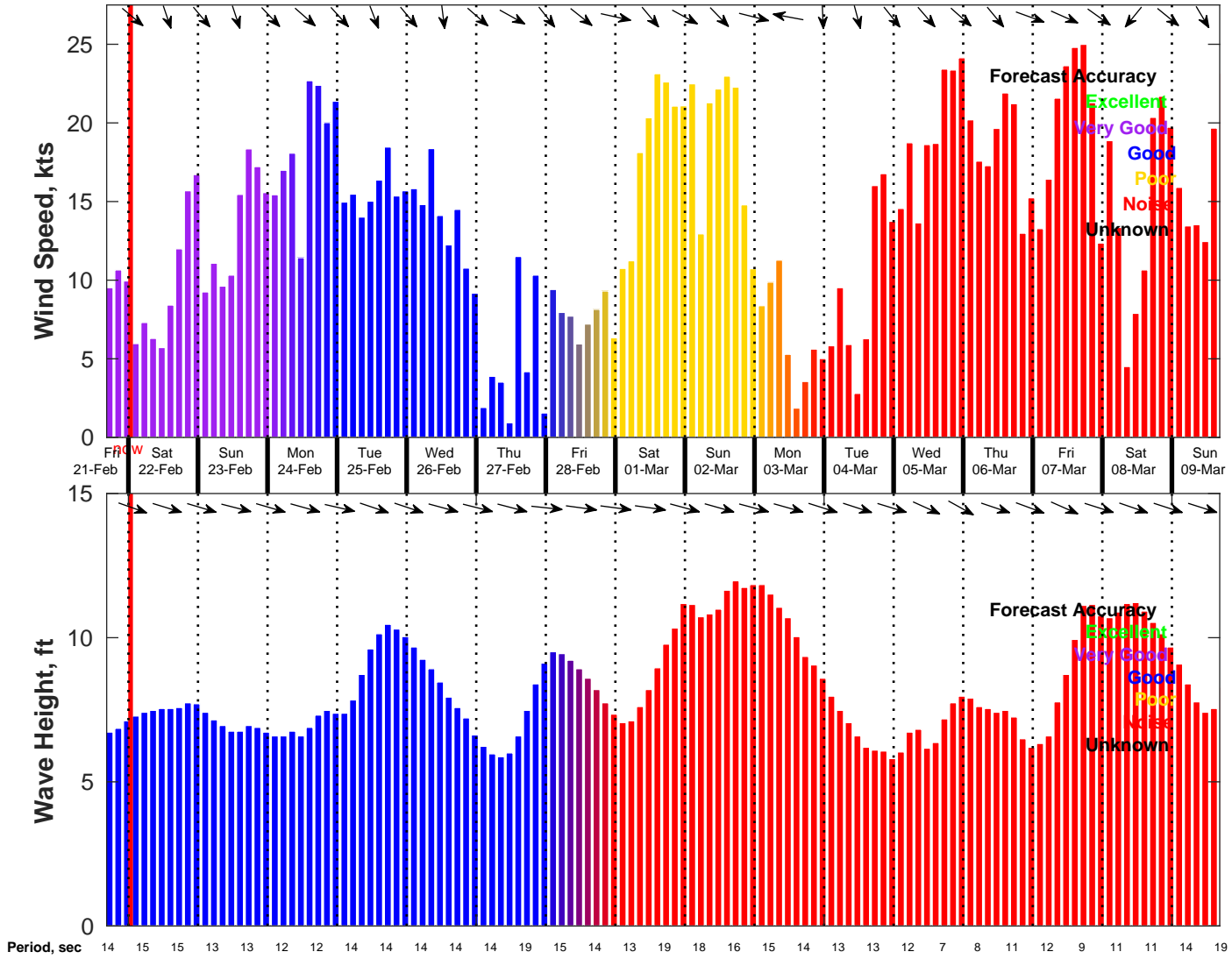
Wind & Wave Forecast for NDBC 46011 from 21-Feb-2025 16:00:00 to 09-Mar-2025 16:00:00
