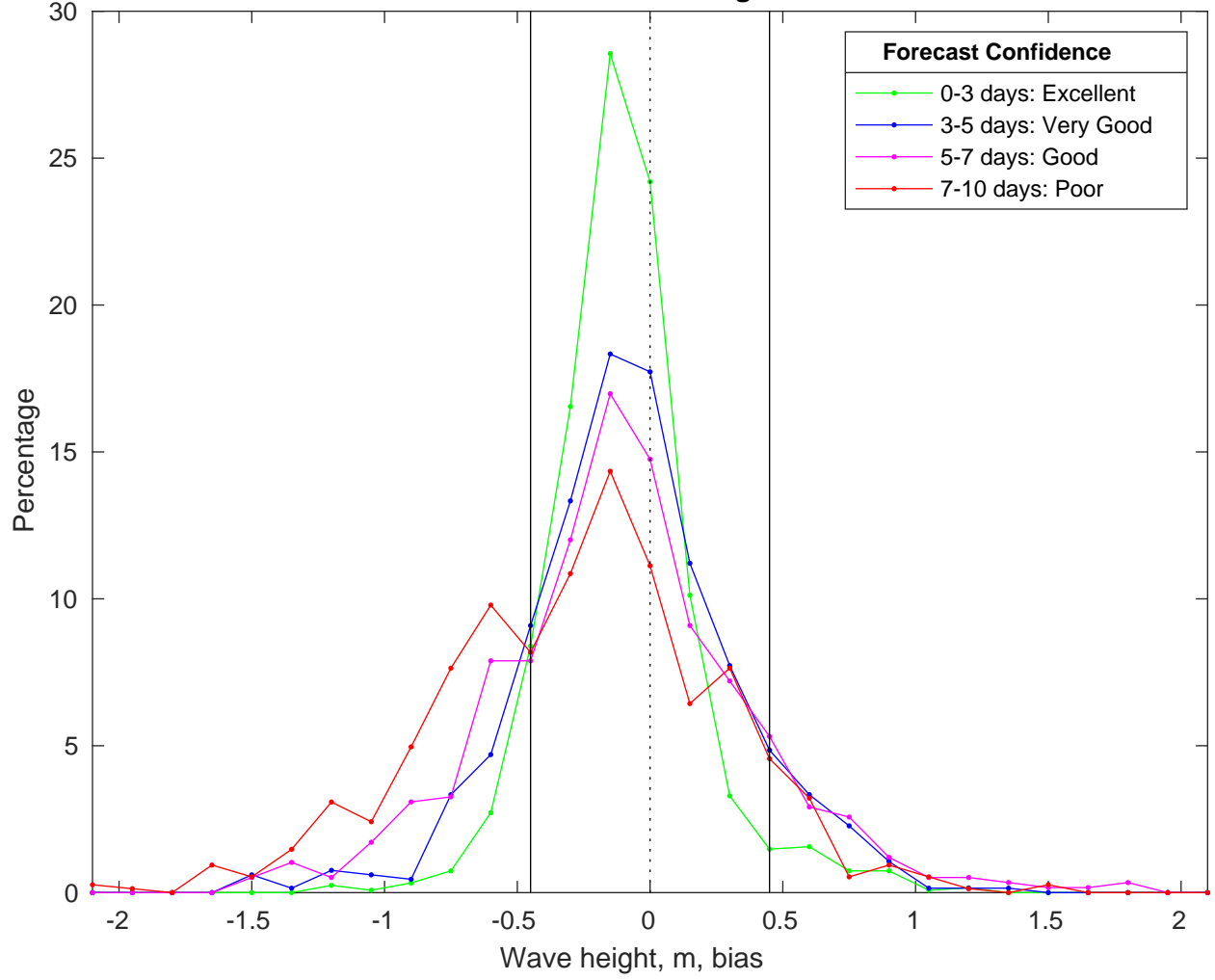
NDBC 46028 vs CMEMS Waves Bias Histogram: 22-Feb-2025
